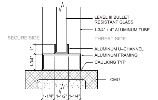
4 ATTORNEY AND IN-CUSTODY WINDOW BASE DETAIL
