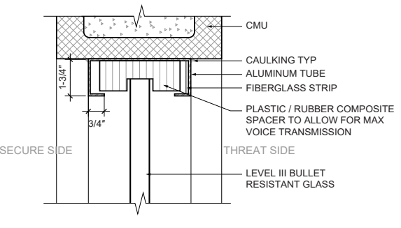
5 ATTORNEY AND IN-CUSTODY WINDOW TOP DETAIL
