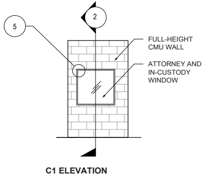
C1 ELEVATION
