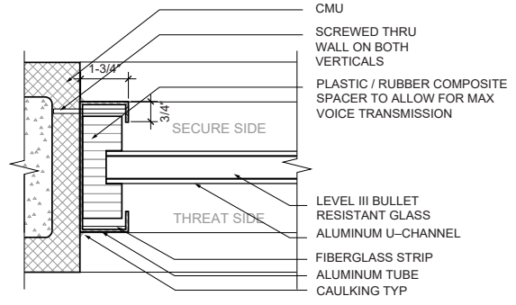
3 ATTORNEY AND IN-CUSTODY WINDOW SIDE DETAIL
