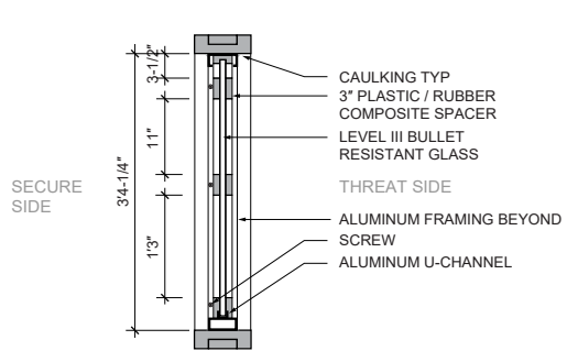
2 ATTORNEY AND IN-CUSTODY WINDOW SECTION
