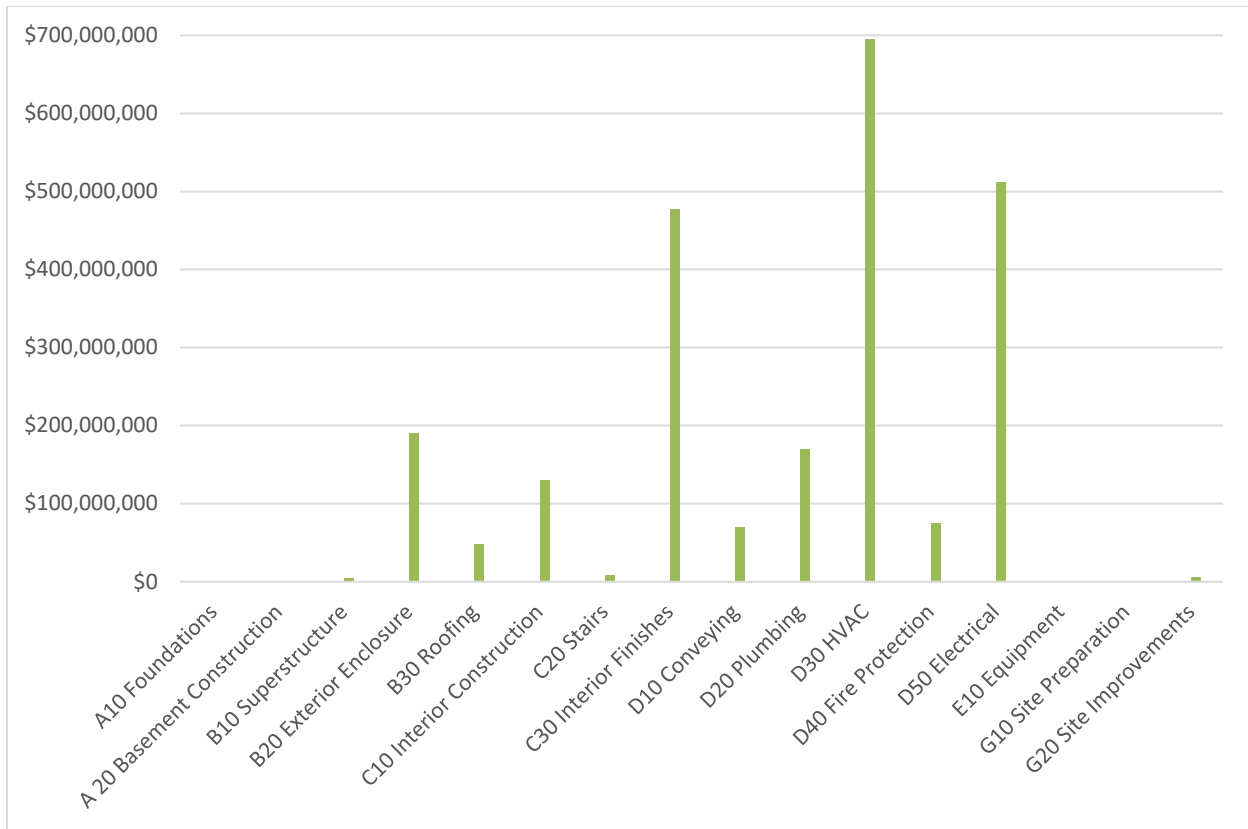
Figure 2: Identified Requests by Building System*
